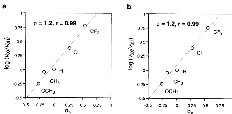
Figure 3. Hammett plots for the DAIB-promoted methylation of benzaldehydes 1a–e . a : the initial rate ratio/ \sigma_p relation with (2 S )-DAIB in 100% ee. b : the initial rate ratio/ \sigma_p relation with ( \pm )-DAIB.
