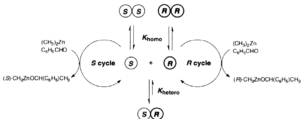
Figure 1. Monomer mechanism.
