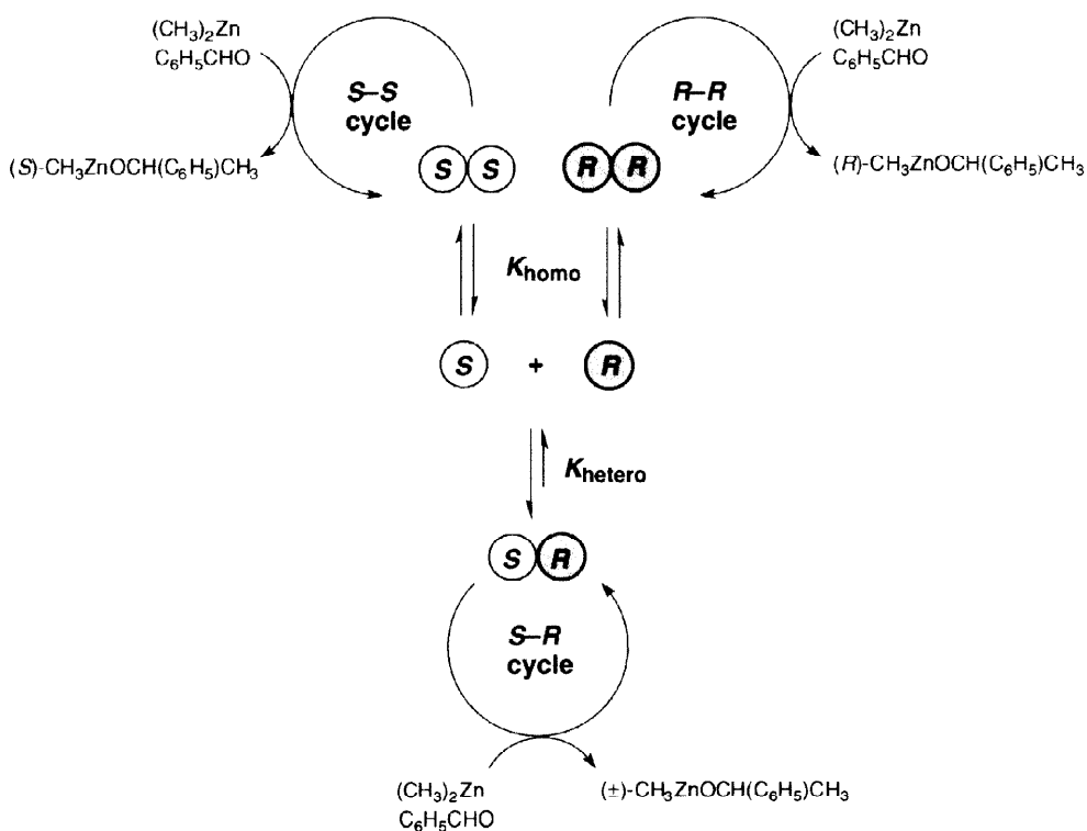
Figure 2. Dimer mechanism.
